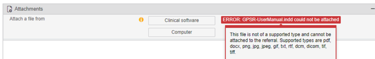
Figure 3: Attachment error
