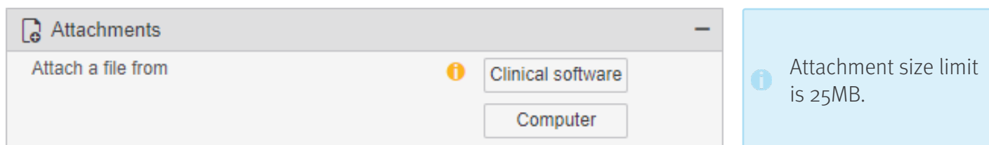
Figure 1: Attachments section
